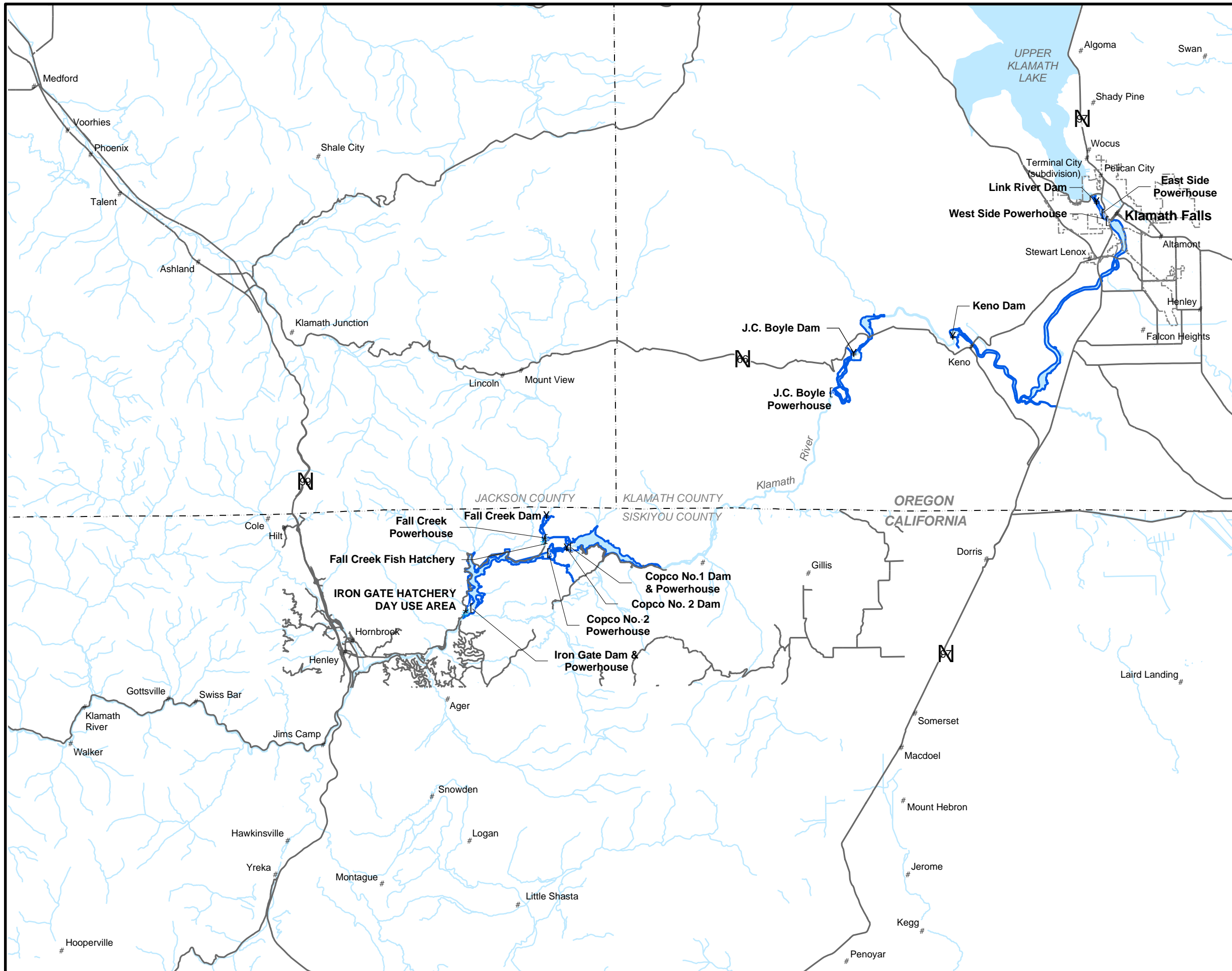
Figure ES1.1-1 Klamath Hydroelectric Project Location
